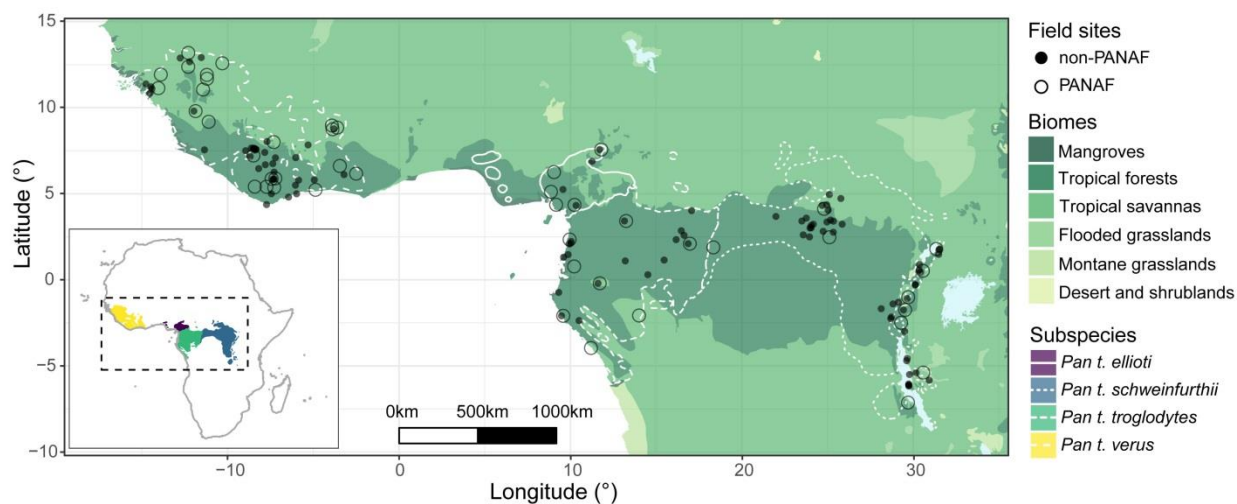
121 122 Fig. 1 Locations of all 144 unique chimpanzee communities for which information on select 123 behaviors was collected for this study. This includes 46 communities from the Pan African 124 Programme (PanAf) and 106 communities for which information was also available from the 125 published literature (non-PanAf). Of these, eight communities had both PanAf and non-PanAf 126 data available. Habitat type represented as biomes modified from the Terrestrial Ecoregions of 127 the World Map 2001.
